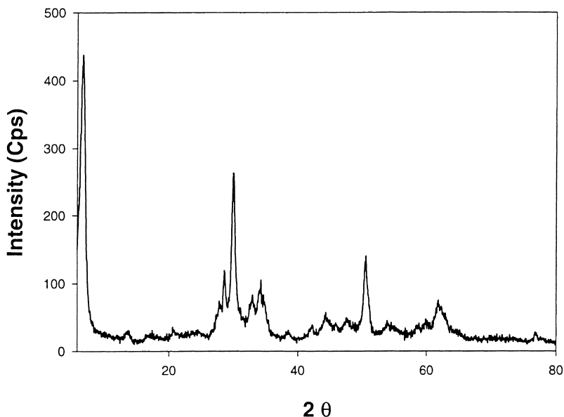
Fig. 7. XRD pattern of NaZ compound.
